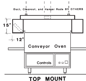
TOP MOUNT
