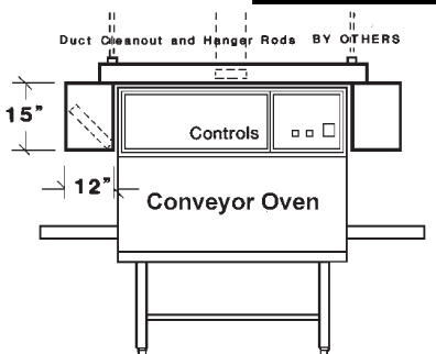
Straddle Mount
