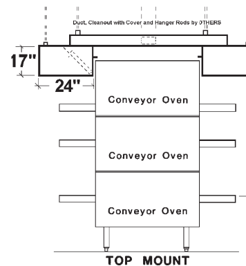
TOP MOUNT
