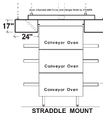
STRADDLE MOUNT
